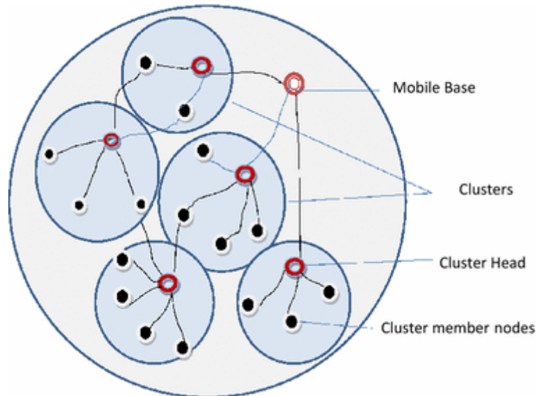
Fig3. Cluster formation
