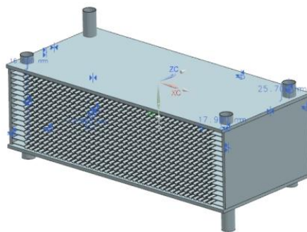
Fig. 2: 3 D model of plate heat exchanger
