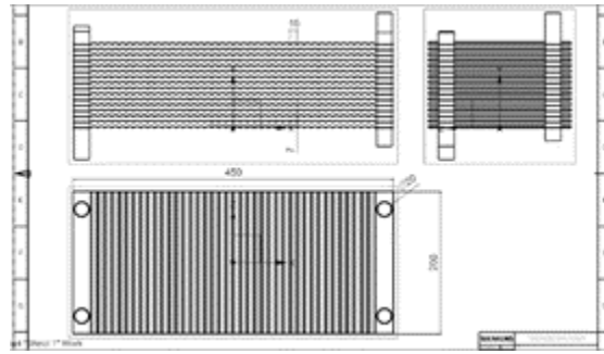
Fig 1: 2 D modeling of corrugated plate
