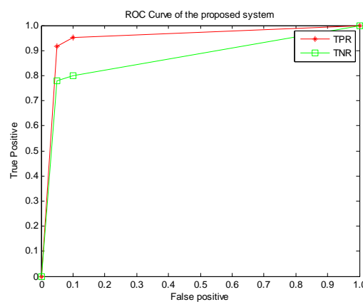
Fig 3. ROC Curve
