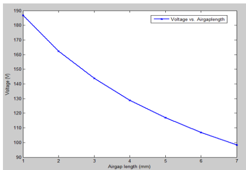
Fig.5 voltage
