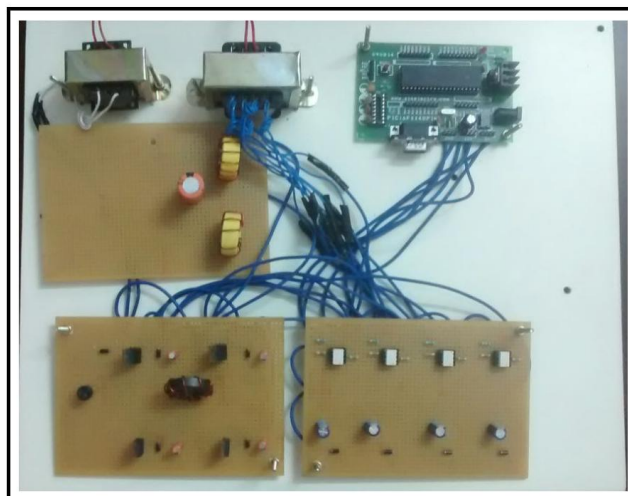
Figure.13 Experimental setup
