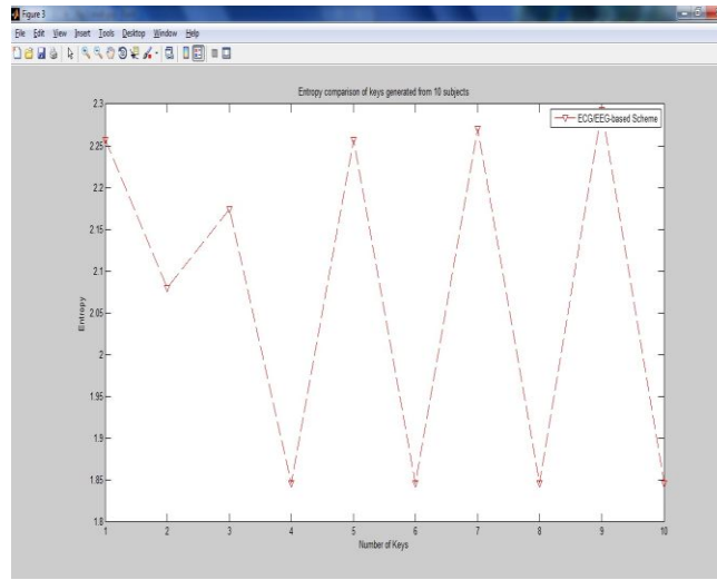
Figure 2: Entropy comparison of keys generated for 10 subjects.
