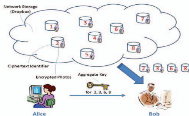
Fig 3-Key Generation
