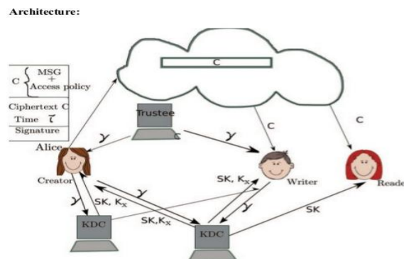
Fig 2-Token Generation
