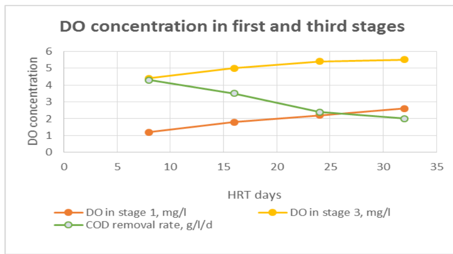
Fig. 9:- DO concentration in first and third stages
