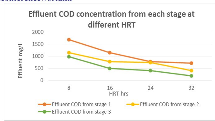
Fig: 6:- Effluent COD concentration from each stage at different HRT
