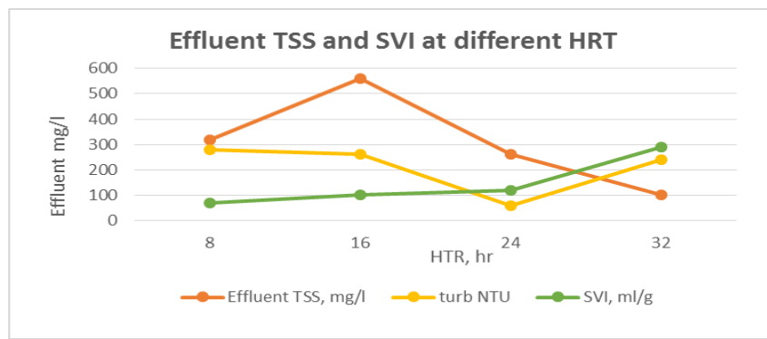
Fig. 5:- Effluent TSS and SVI at different HRT
