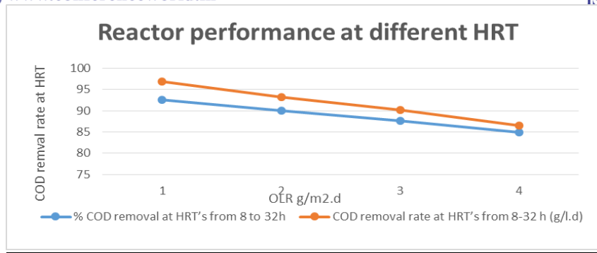
Fig. 4:- Reactor performance at different HRT
