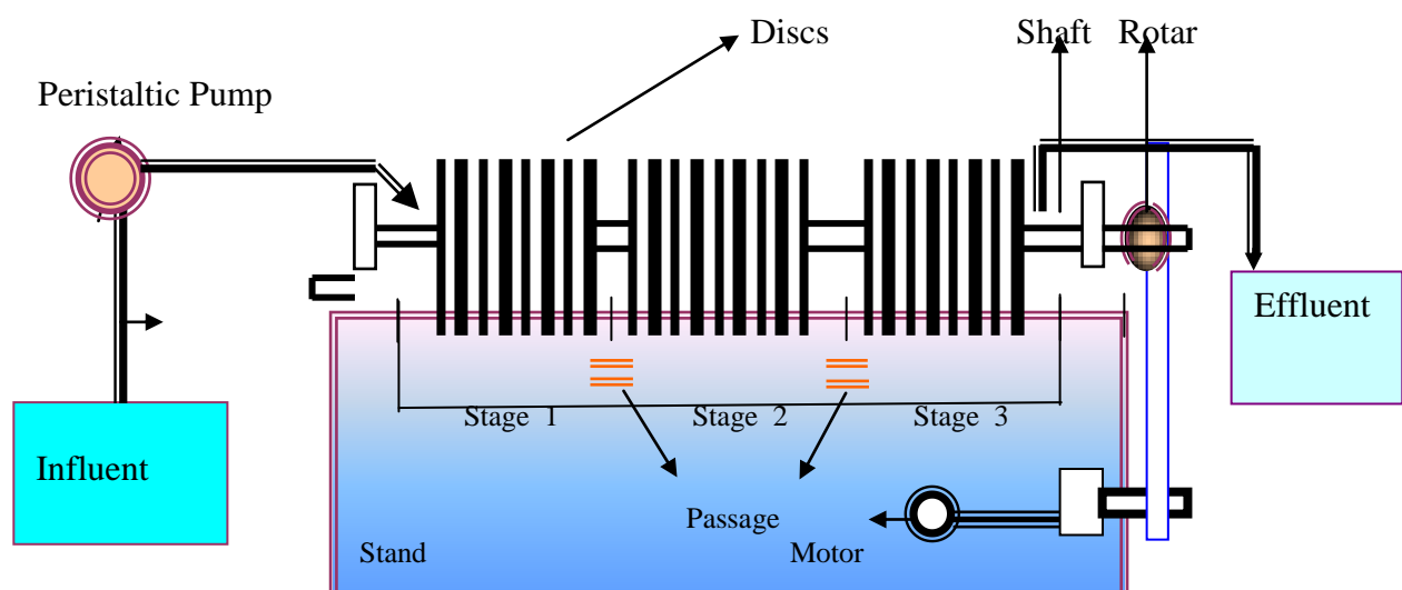
Fig 1: Sketch of the Experimental Set-up of RBC Bioreactor.
