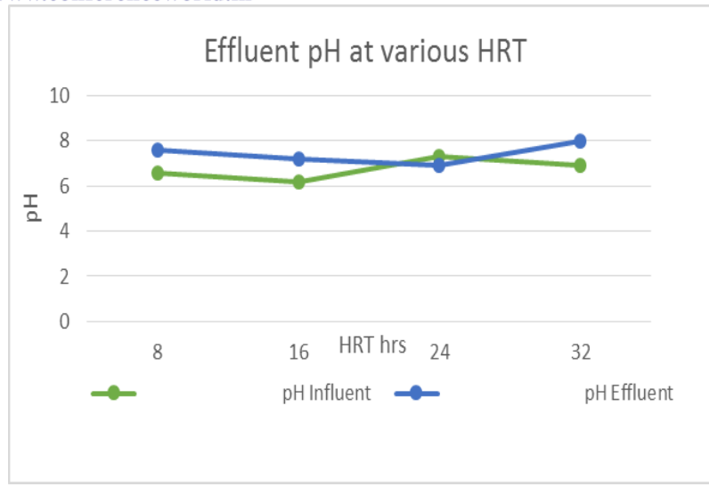
Fig. 8:- Effluent pH at various HRT
