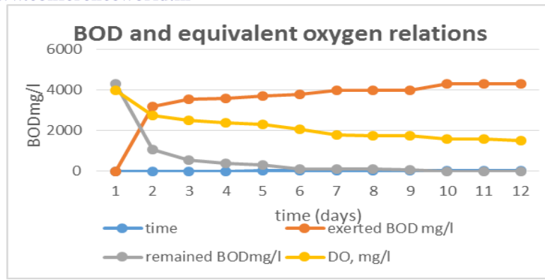
Fig. 2:- BOD and equivalent oxygen relations
