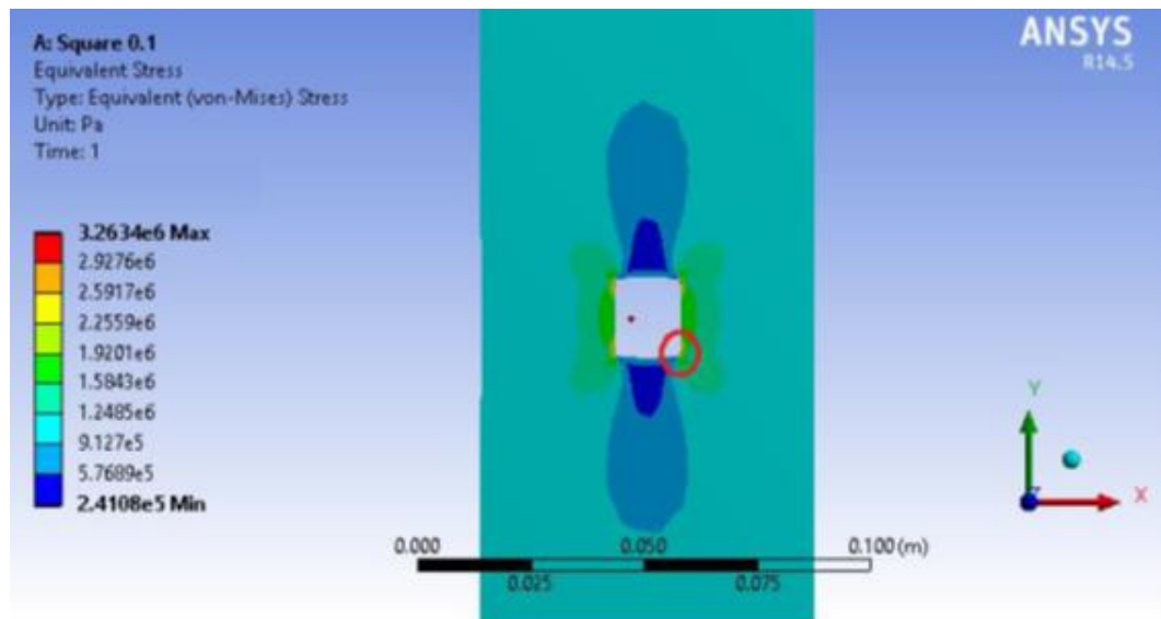
Fig.8. Stress Contour of Plate with Square Cutout ( r/R = 0.1 )
