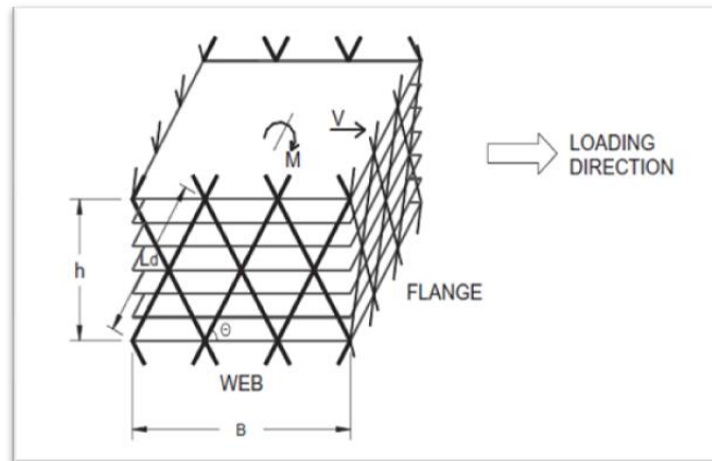
Fig.1.1.1. Diagrid structure
