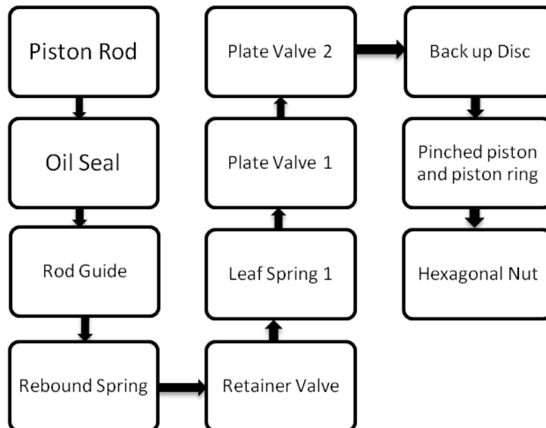
Fig. 2.1: Operational Sequence of Piston Rod Assembly
