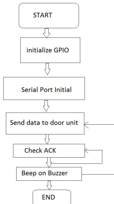
Figure 11 flowchart of watch unit
