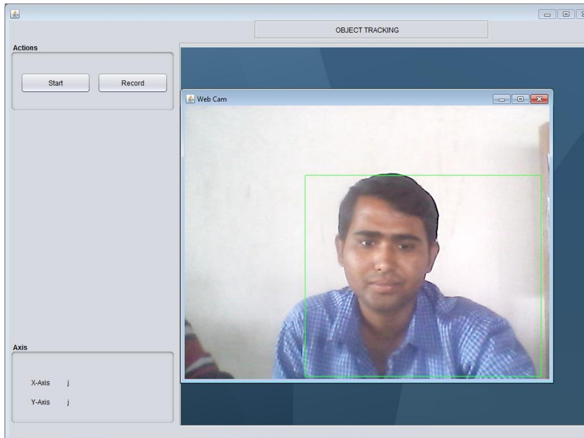
Fig.5 Object Detection
