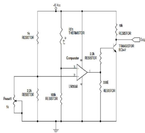
Fig 5. Circuit diagram for temperature sensor
