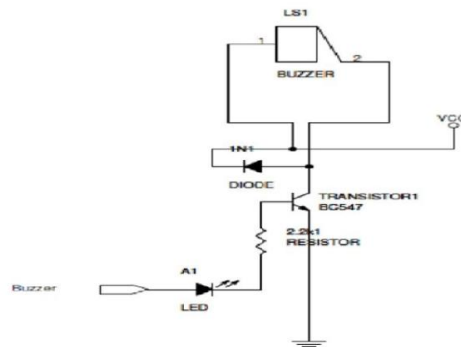
Fig 4. Buzzer circuit
