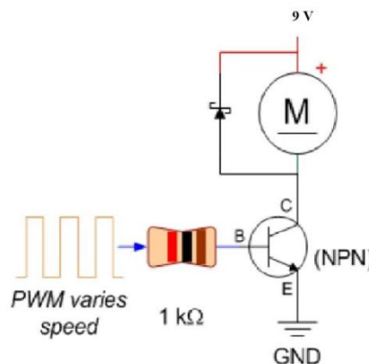
Fig 3. Driver circuit
