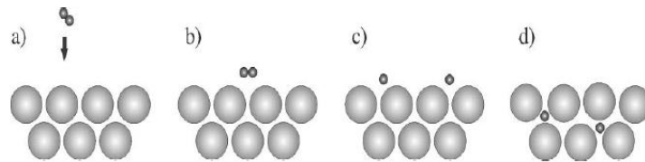
Figure 2.2.1 Movement of hydrogen molecules
