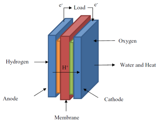
Figure 1.2 The operating principle of a fuel cell.
