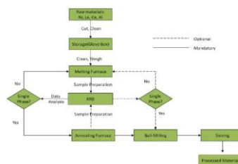
Figure 3.1 Preparation of Metal Hydride alloys
