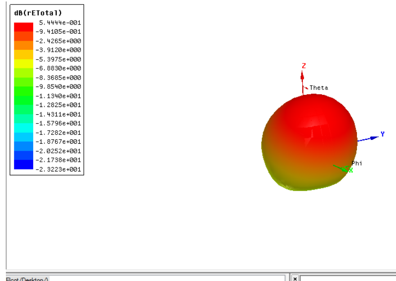
Fig. 4. Gain of microstrip patch antenna.
