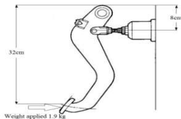
Fig. Dimension and Force applied
