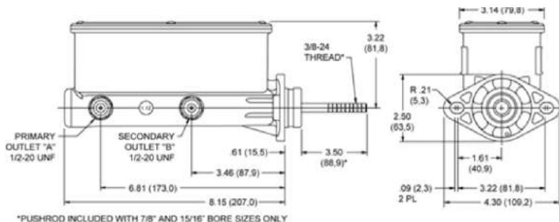
Dimensions of brake cylinder
