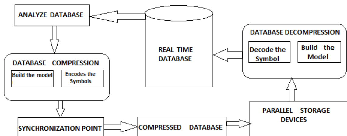
Fig 1:-Structure of Database Compression and Decompression
