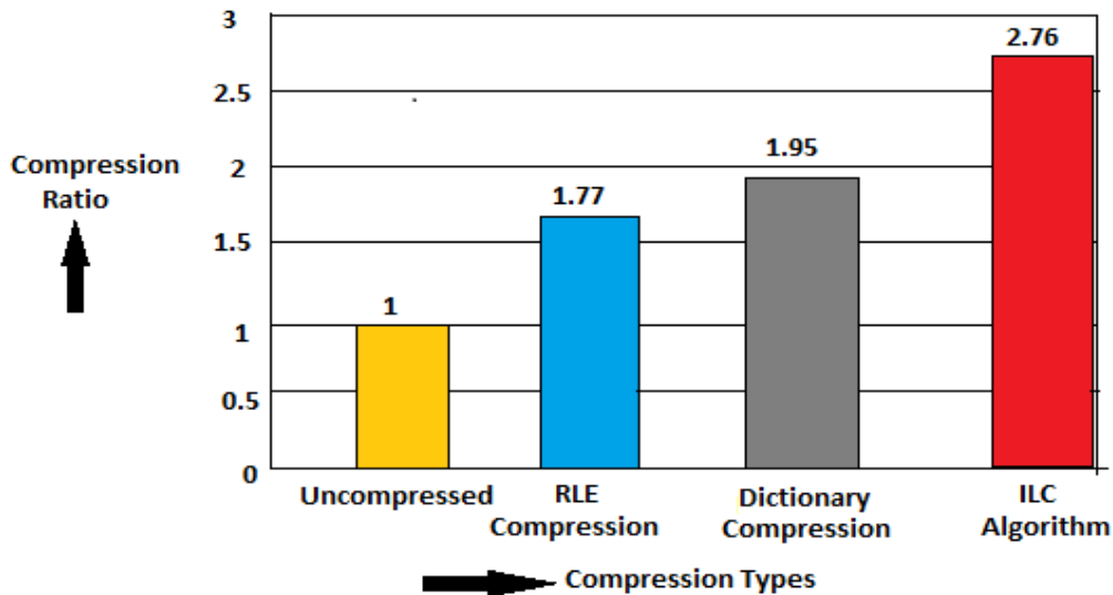
Fig. 2 Compression Types vs Compression Ratio
