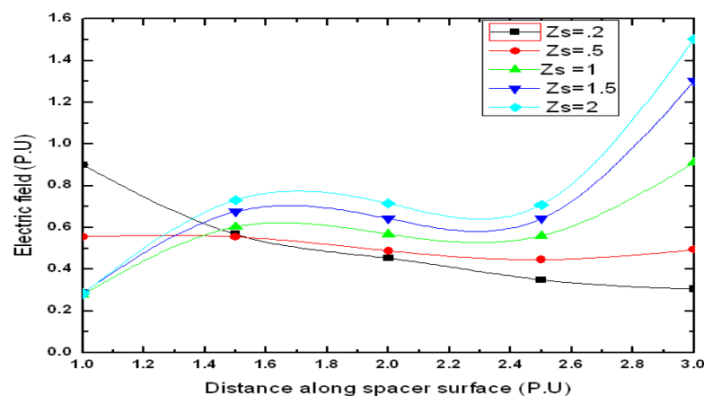
Fig. (2) Effect of Z_s on the electric field distribution along the spacer surface
