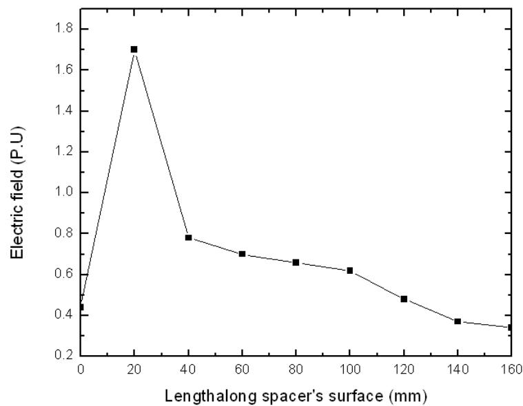
Fig. (9) Electric field distribution along concave side of initial shape at r=4mm
