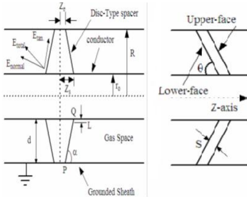
(a) Disc spacer
