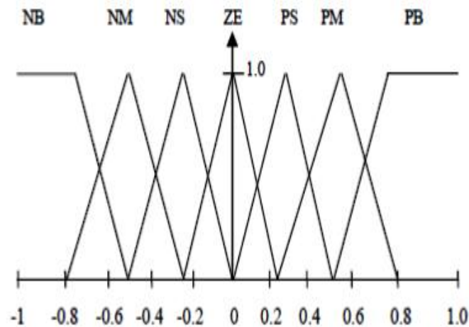
Fig.4. Membership Function for Output Variable Change in Control Signal, 'u'
