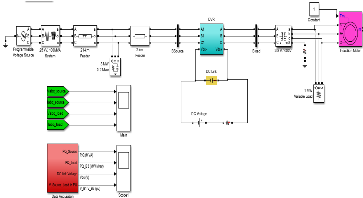
Fig.5 Simulation Diagram
