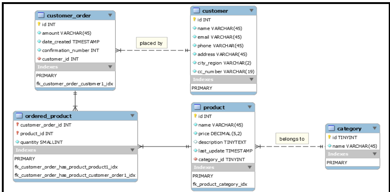
Figure 4. Entity relationship diagram of Paragon
