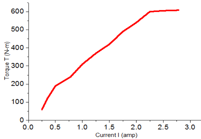
Fig 7. Torque variation with current
