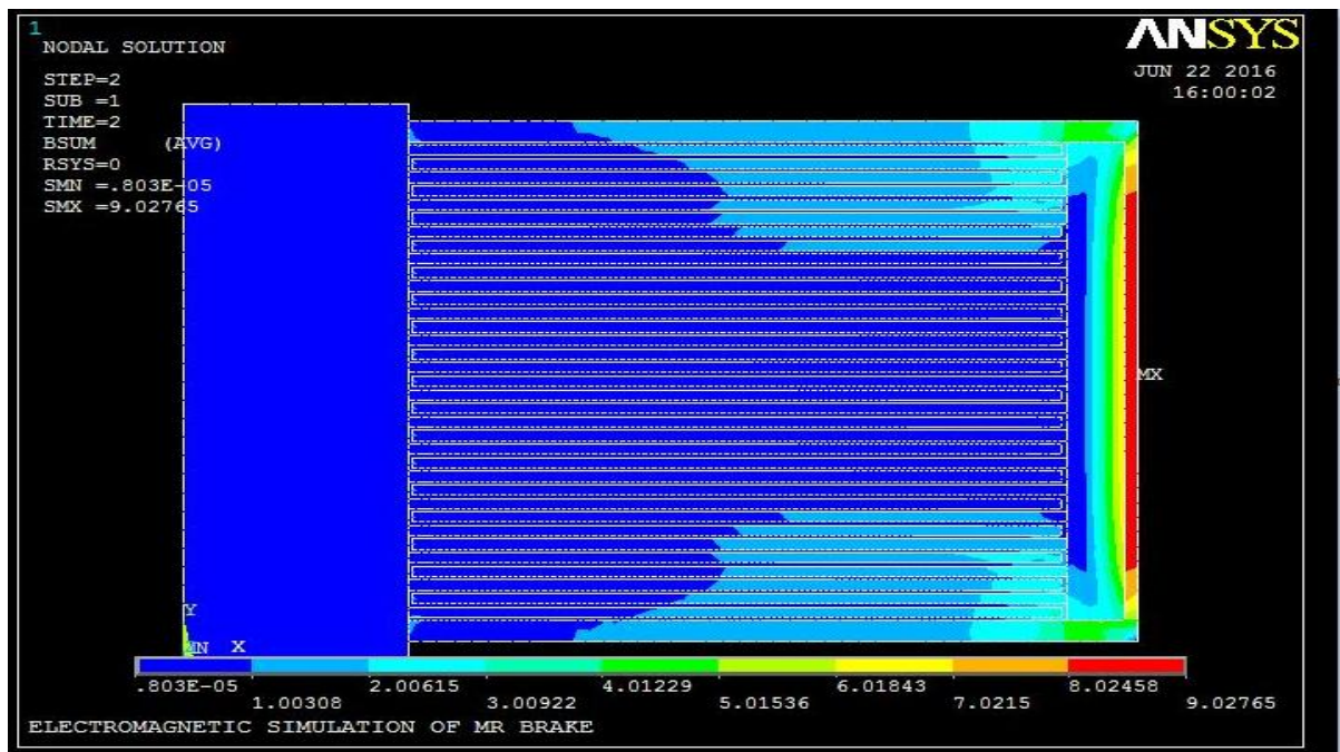
Fig 6. Magnetic flux density by nodal plot.
