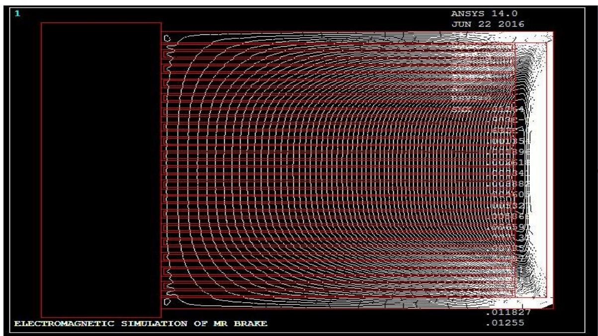
Fig 4. Two dimensional flux lines.
