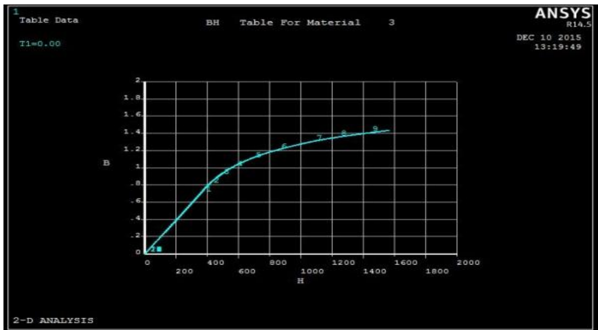
Fig 3. B-H curve for Finite element analysis.
