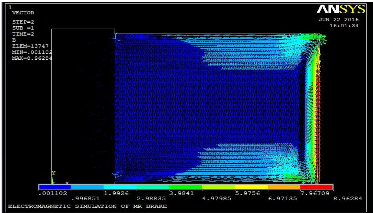
Fig 5. Magnetic flux density by vector plot.
