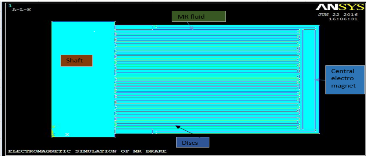
Fig 2. Two dimensional axi-symmetric model of Multidisc MR Brake.
