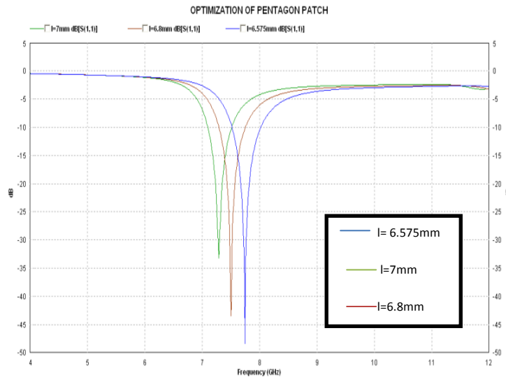
Fig.2.Optimization of pentagon patch
