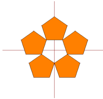
Fig.3. Fractal geometry
