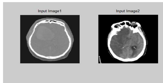
Figure10: Input Images
