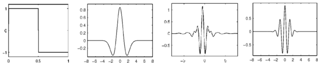
Figure1:- Wavelet family examples, from left to right: Haar, Mexican Hat and Morlet.
