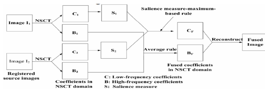
Figure 7:- Framework
