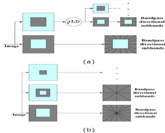
Figure6:-Decomposition framework of contourlet transform and NSCT.
