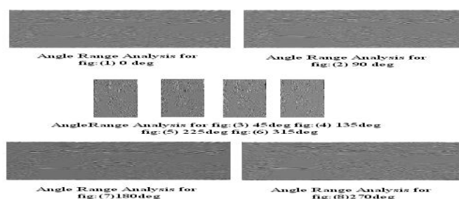
Figure9:- Discrete Curvelet Transform Process
