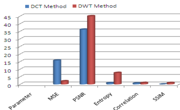
Figure12:- Comparison graph for DCT and DWT Methods
