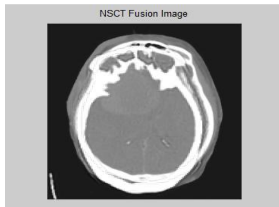
Figure11:- Fusion Image
