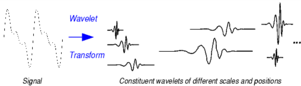
Figure2:- Wavelet analyses represent the signal as combination of scaled and shifted mother wavelets.
