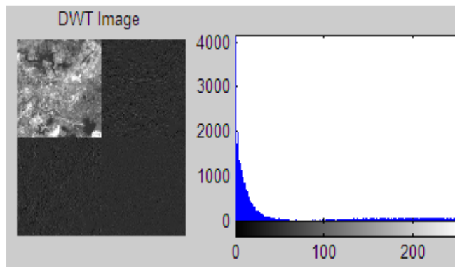
Figure5:-Example of DWT Image and Histogram Image
