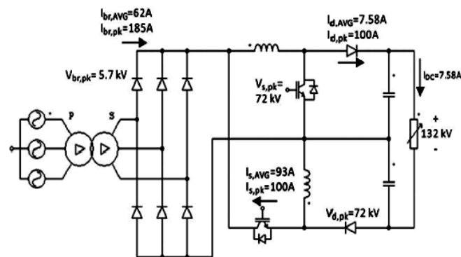
Fig 3. Multiple module series hybrid converter
