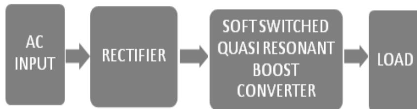
Fig 7. Block diagram of soft switched multiple module quasi resonant boost converter
