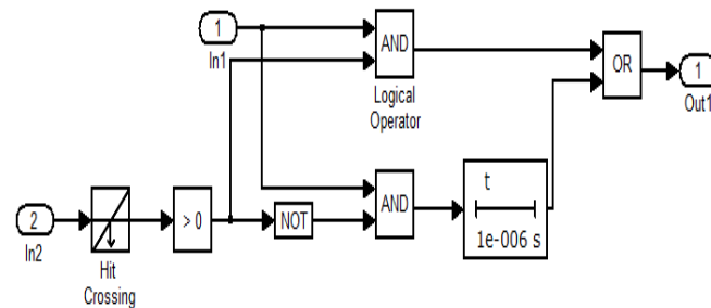
Fig 10. Sub system component of Soft switched multi module quasi resonant boost converter
