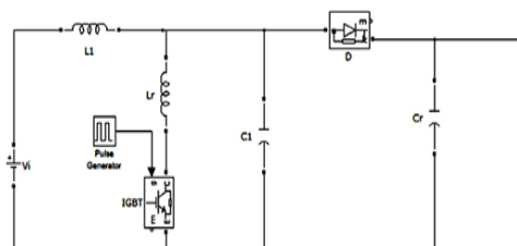
Fig 8. Quasi-resonant Boost Converter
