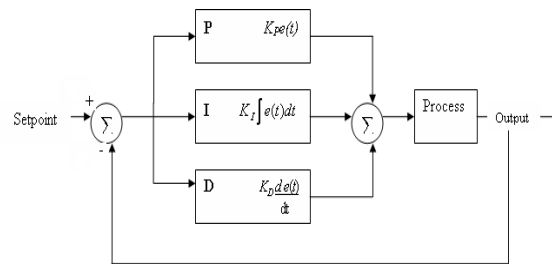
Block Diagram of PID controller
