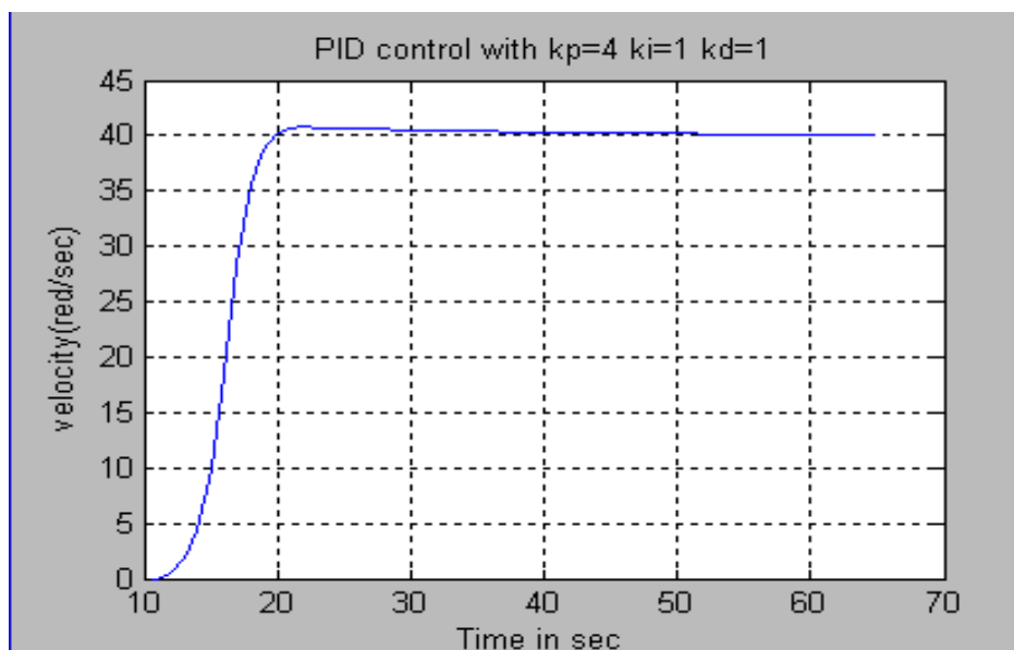
PID controller with: K_p=4, K_i=1 and K_d=1
