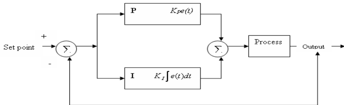
Block Diagram of PI controller
