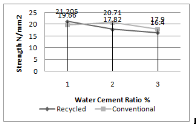
Figure 4: Characteristic strength (MPa) at 28 days
