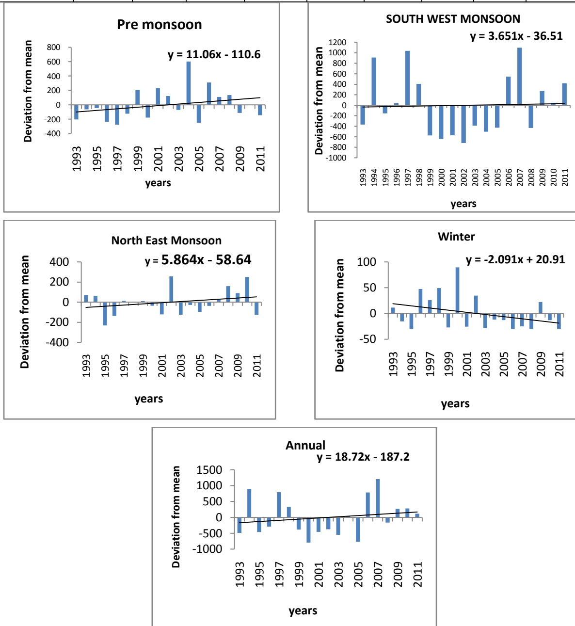
Figure 2: Rainfall Trend of Ambalavayal Station
