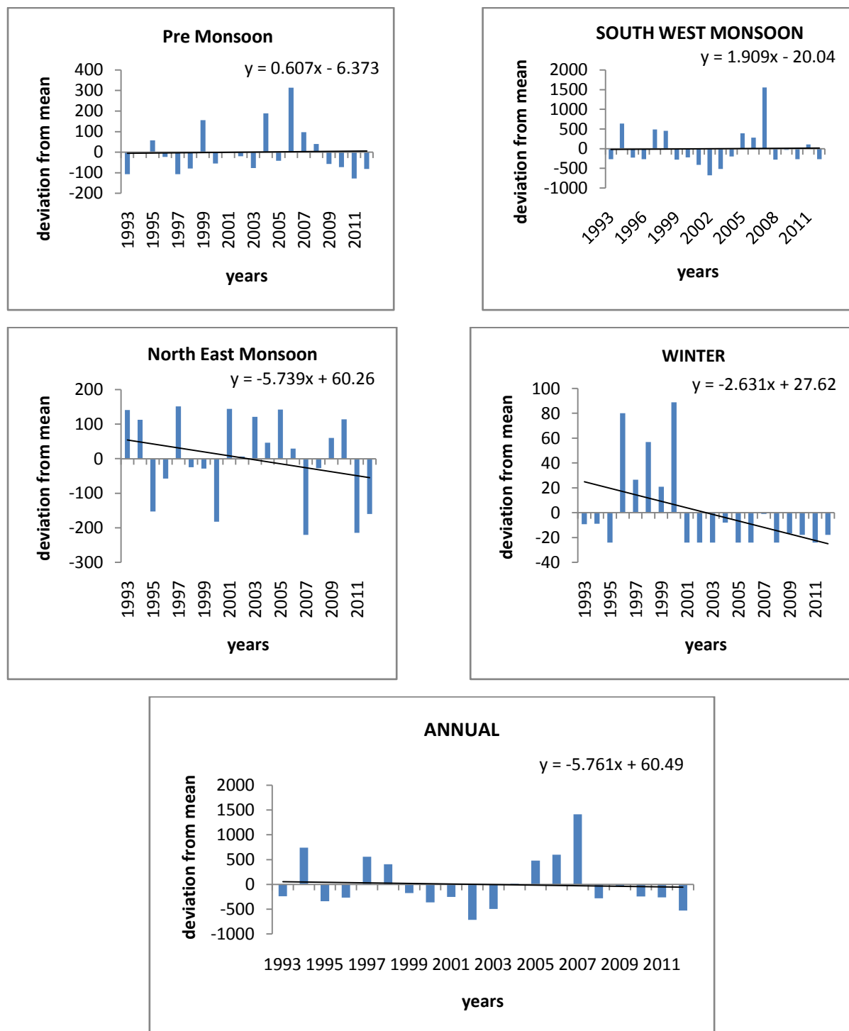
Figure 5: Rainfall trend of Nilambur station
