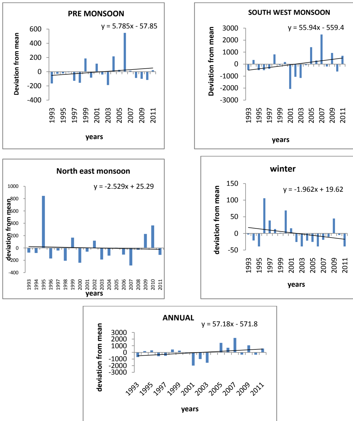
Figure 3: Rainfall Trend of Kalladi Station
