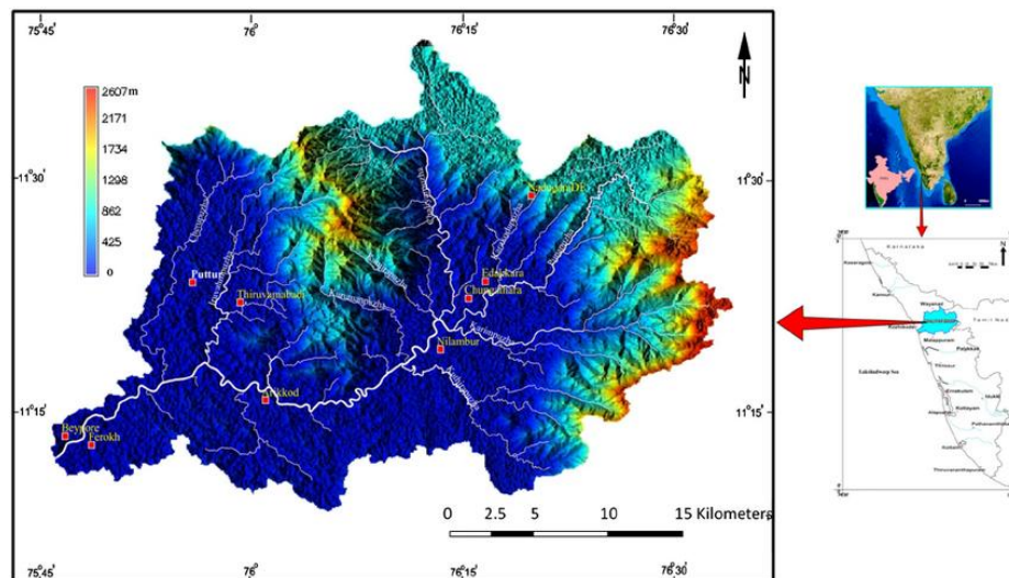
Figure 1: Digital elevation model (DEM) aspect map of the Chaliyar River drainage basin.
