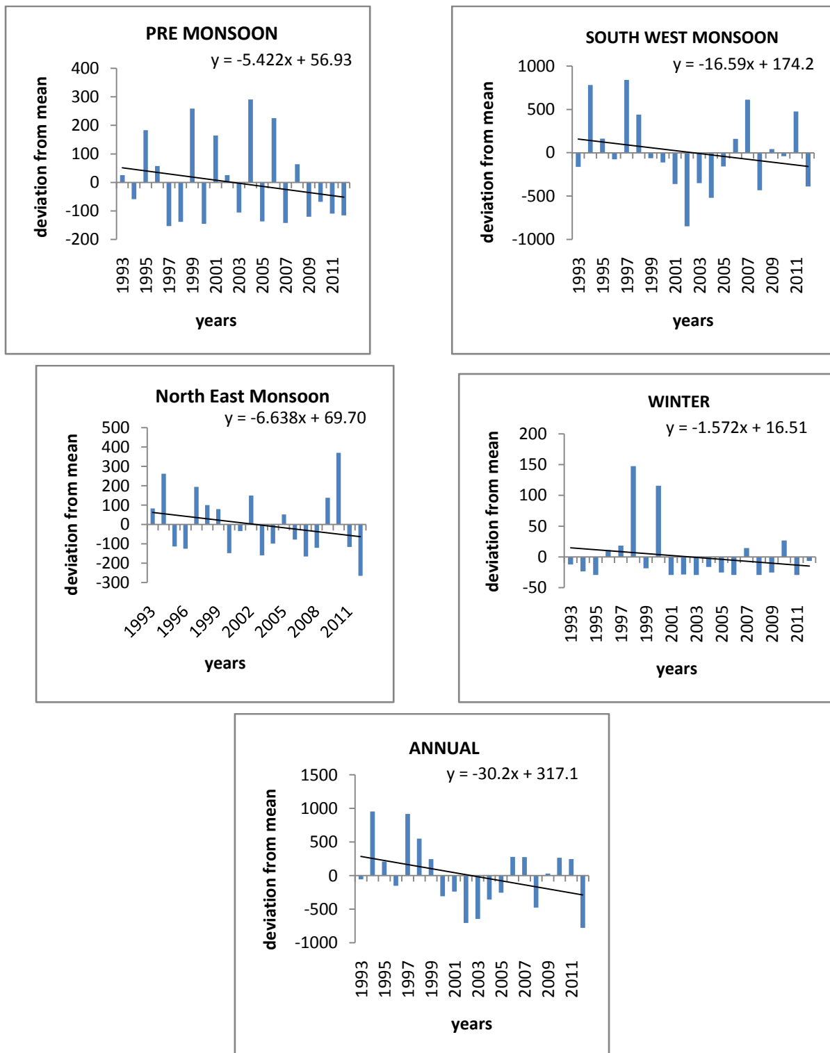
Figure 4: Rainfall trend of Manjeri station
