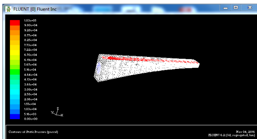
Fig. 7 Pressure Contour1
