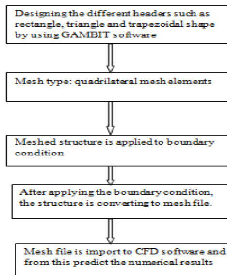
Fig. 3 Flow Chart for Methodology
