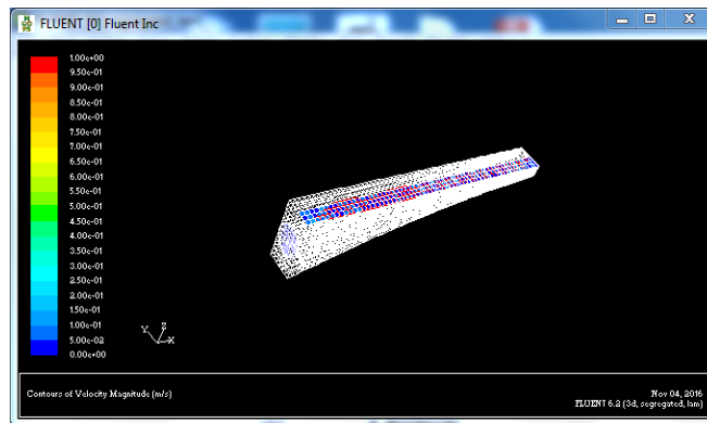
Fig. 9 Velocity Contour1
