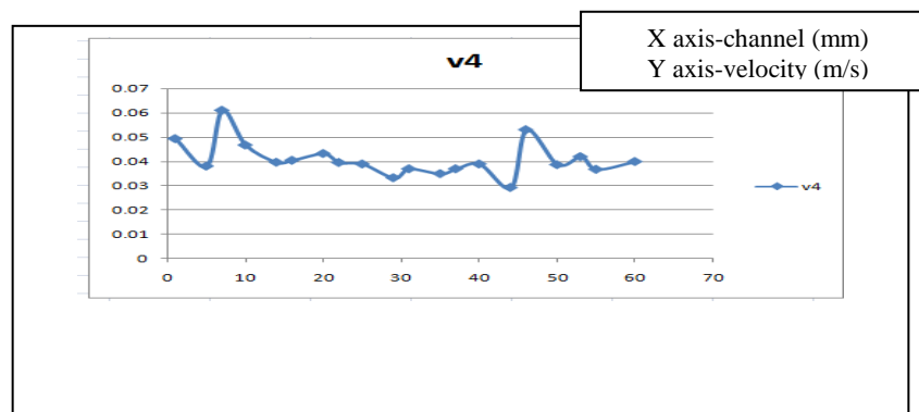
Fig. 11 Waveform for Rectangular Header
