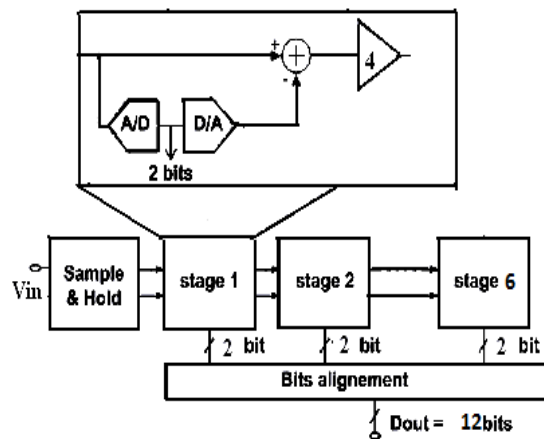
Figure 2 Block diagram of proposed pipeline ADC
