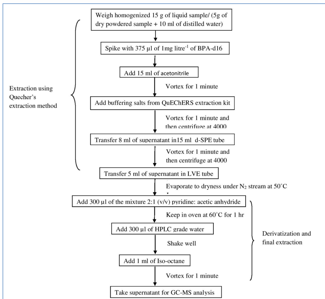
Fig.1 Scheme of sample preparation for BPA analysis
