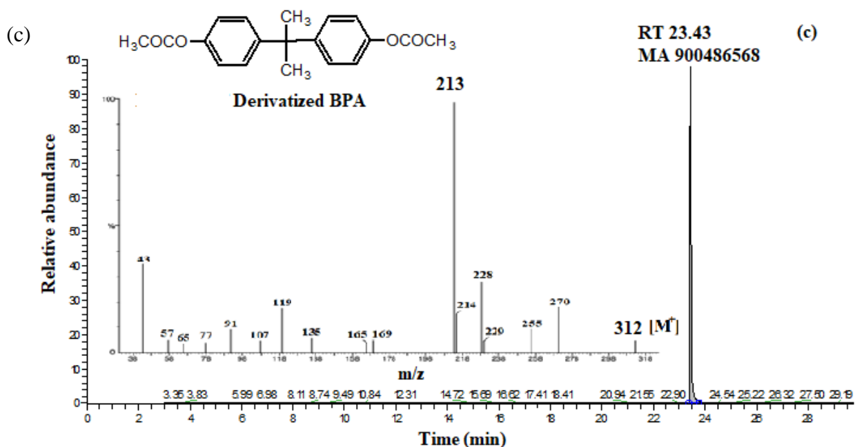
Fig.2 (c) TIC of BPA derivatized 100 ppm std solution after extraction by method 2 (along with full mass spectra of derivatized BPA at RT 23.43)
