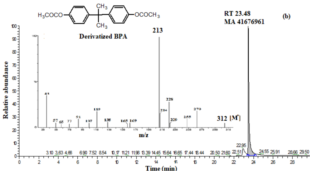
Fig.2 (b) TIC of BPA derivatized 100 ppm std solution after extraction by method 1 (along with full mass spectra of derivatized BPA at RT 23.48)
