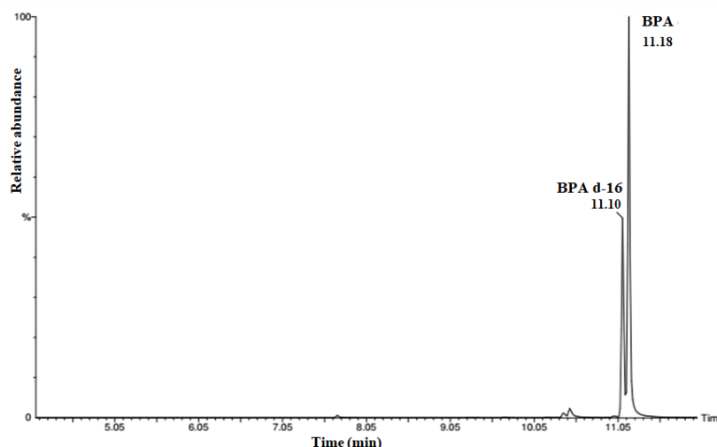
Fig.3 (a) TIC of std solution of 25 ng g -1 of BPA-d16 & 25 ng g -1 using 5 channels (213, 224, 228, 270 and 312) m/z
