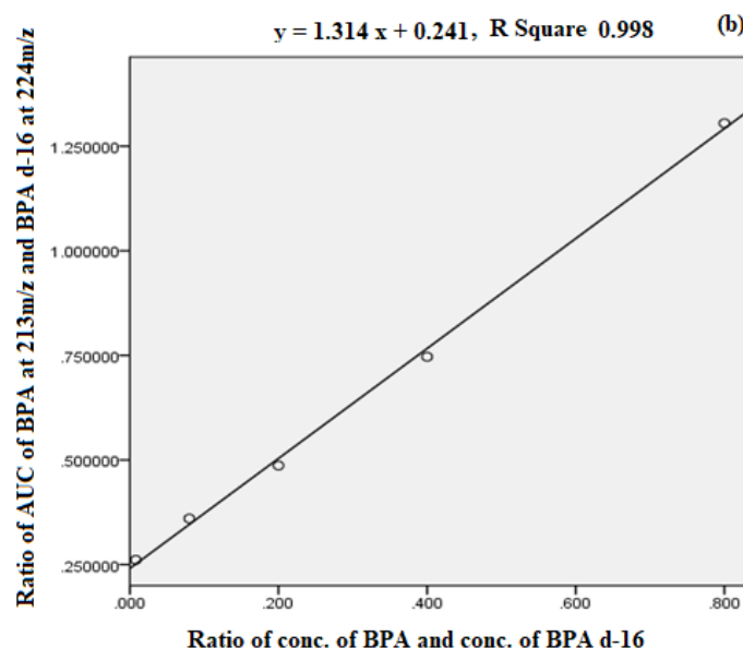
Fig.3 (b) Linear standard calibration curve of BPA by using BPA d-16 as an internal standard
