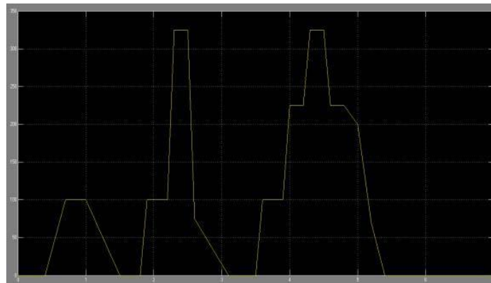
Fig.8. Drive cycle with the maximum vehicle speed of 25kmph( corresponding motor speed of 330rpm)
