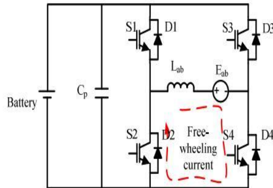
(b) When S4 only is closed (State-I) for free-wheeling mode
