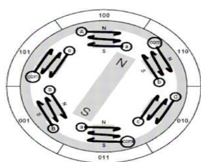
Fig 1. Permanent Magnet BLDC motor
