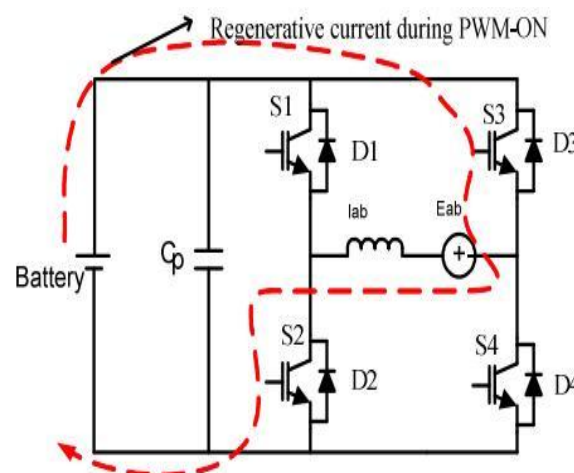
(a) When S2 and S3 are closed with PWM-ON (State-I) for regenerative mode
