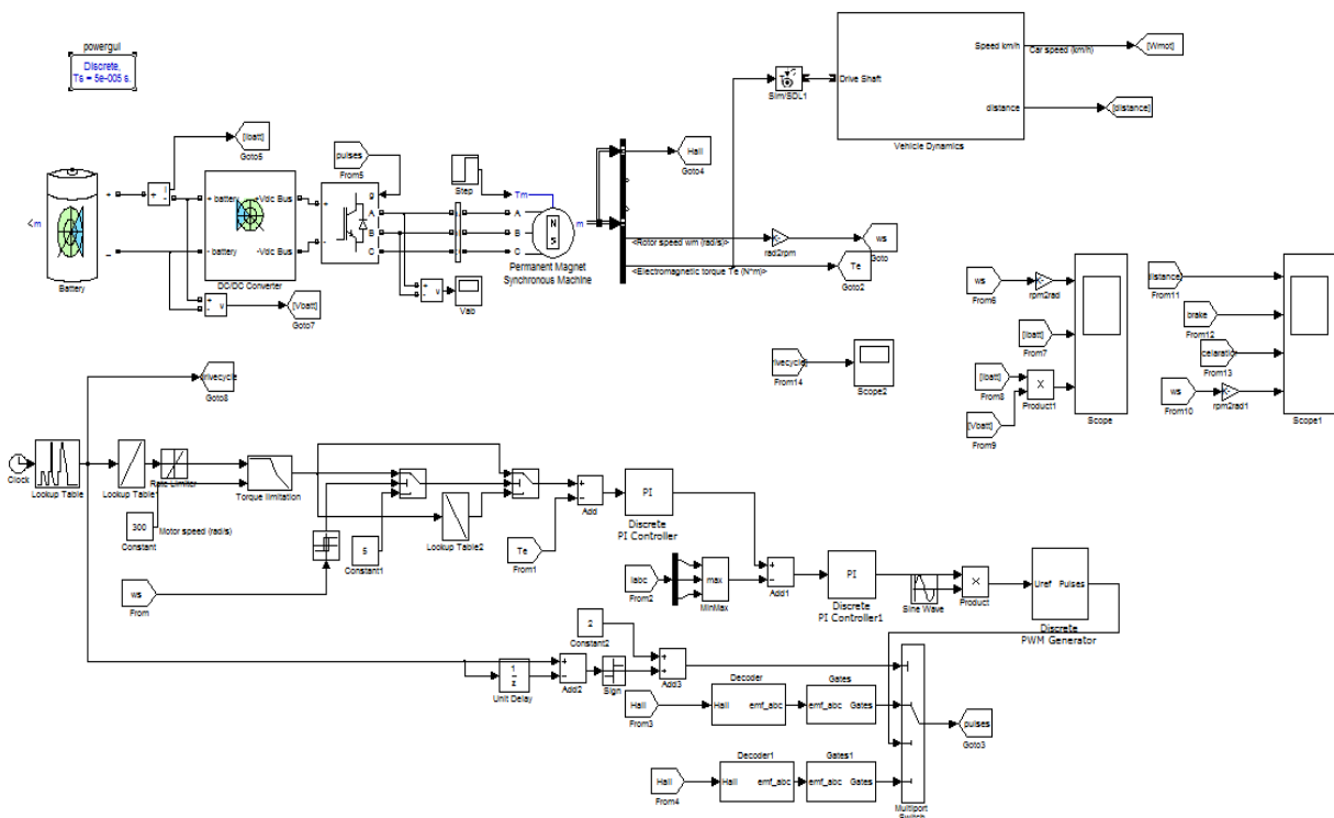
Fig.7. Simulink model of the 3-phase PM BLDC motor during the regenerative mode
