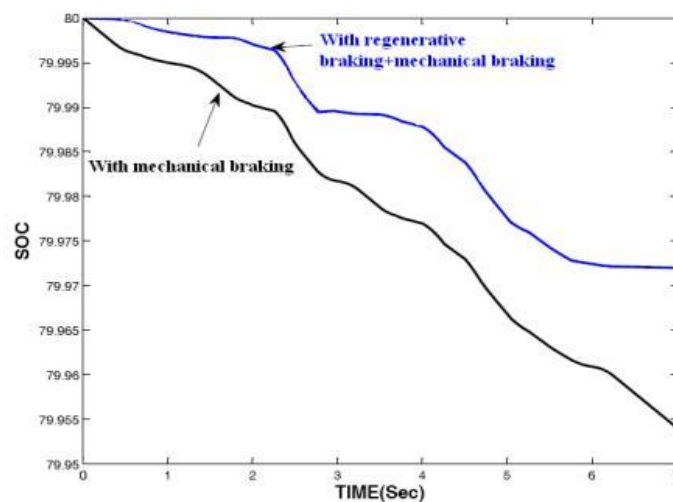
Fig.11. Comparison of SOC for different braking methods
