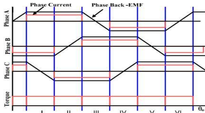
Fig. 3. Ideal back-EMF, phase current and developed torque profiles in a 3-phase PM BLDC motor
