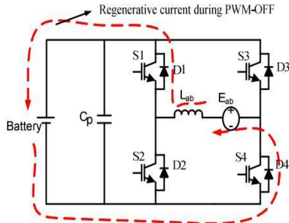
(b) When S2 and S3 are open with PWM-OFF (state- I) for regenerative mode
