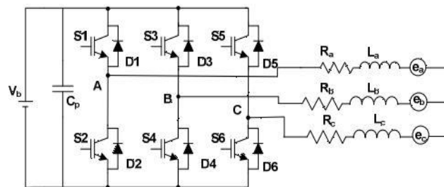
Fig. 2 Equivalent circuit of an inverter driven 3-phase PM BLDC motor
