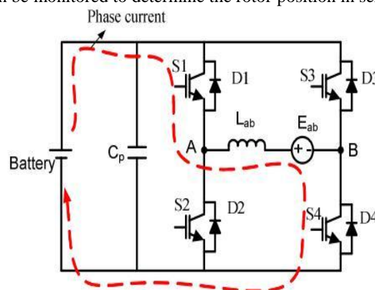
(a) When S_1 and S_4 are closed with PWM-ON (State-I) for motoring mode
