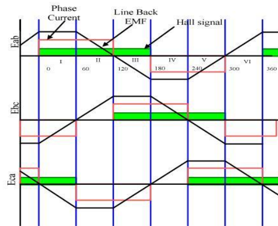
Fig.5. Regenerative braking strategy in a 3-phase PM BLDC motor using the line back-EMF
