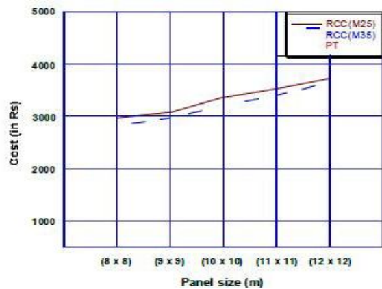
Fig.12 Cost comparison plot of RCC and PT flat slabs
