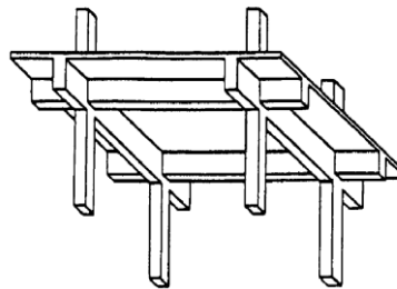
Fig. 8 Two way beam slab
