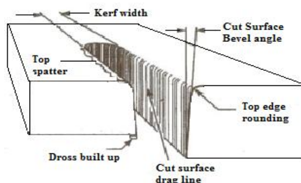
Fig.2 Quality Characteristics of Plasma Arc Cutting Process
