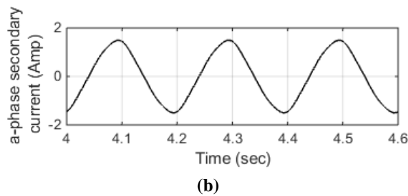
Fig.6: a-phase secondary current under (a) normal and (b) harmonic condition
