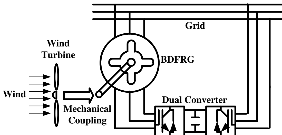
Fig. 1: Local grid connected BDFRG
