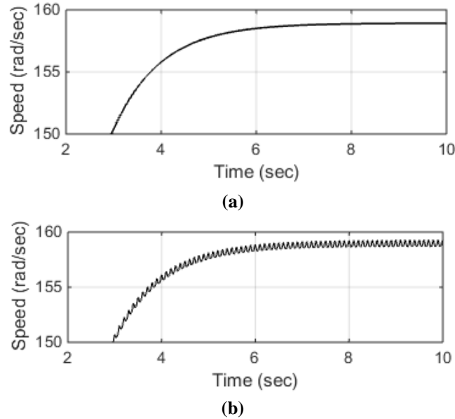
Fig.9: Rotational speed under (a) normal and (b) harmonic condition
