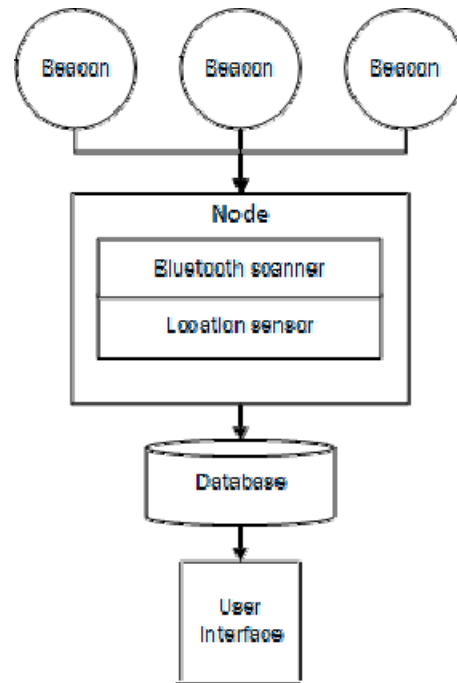
Fig. 1. Smart School Tracking Architecture
