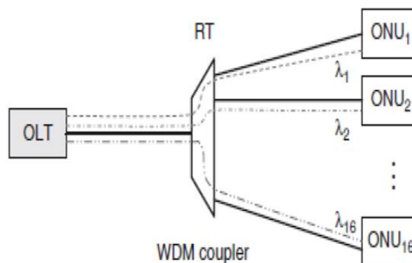
Figure 3- WDM PON [4]
