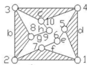
Fig.1: Eight -Link, Single DOF K C
