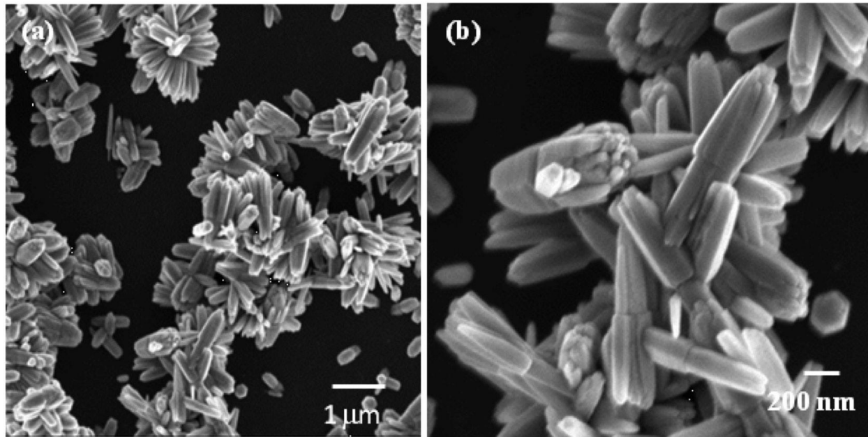
Fig 2: SEM images of ZnO Nanostructures (a) 10 kX (b) 30 kX (Reproduced from Ref.12)
