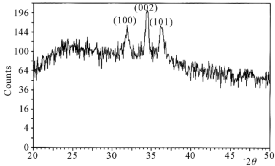
Fig 4: XRD pattern of ZnO Nanostructures (Reproduced from Ref.14)
